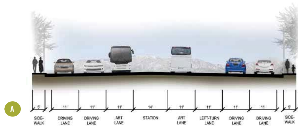
STATION CROSS SECTION AT WYOMING
