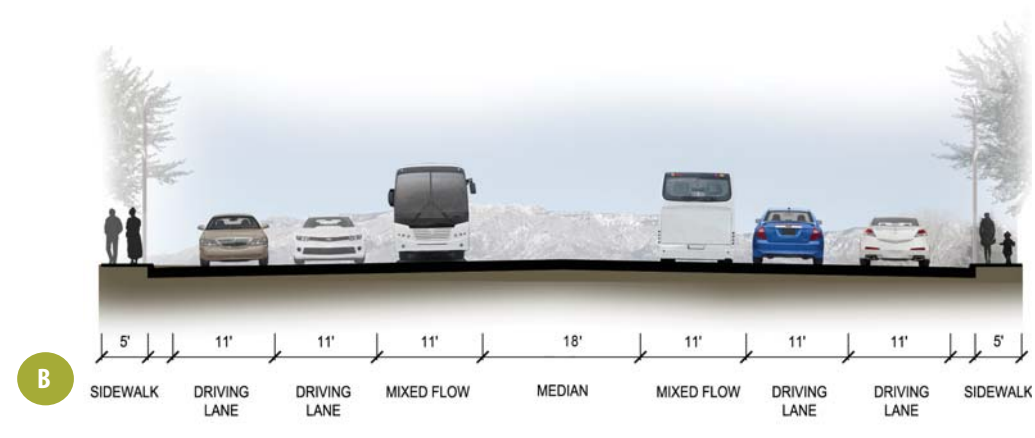
CROSS SECTION
